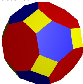
Truncated Cuboctahedron Truncated Icosidodecahedron a.k.a. Great Rhombicuboctahedron, Great Rhombicosidodecahedron
