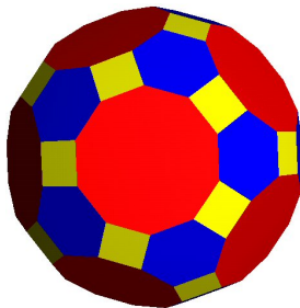
Truncated Cuboctahedron Truncated Icosidodecahedron a.k.a. Great Rhombicuboctahedron, Great Rhombicosidodecahedron
