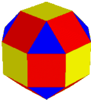
Rhombicuboctahedron
