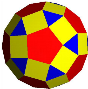
Rhombicosidodecahedron
