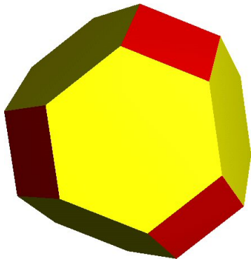
Truncated Octahedron
