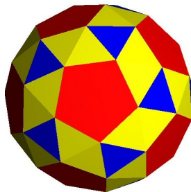
Snub Dodecahedron
