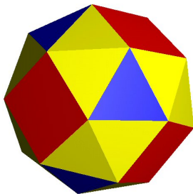
Snub Cube
