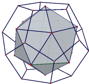
Regular Icosahedron
