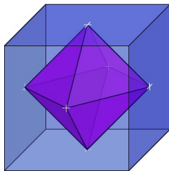
Regular Octahedron
