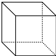
Cube (Regular Hexahedron)
