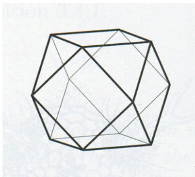
Cuboctahedron
